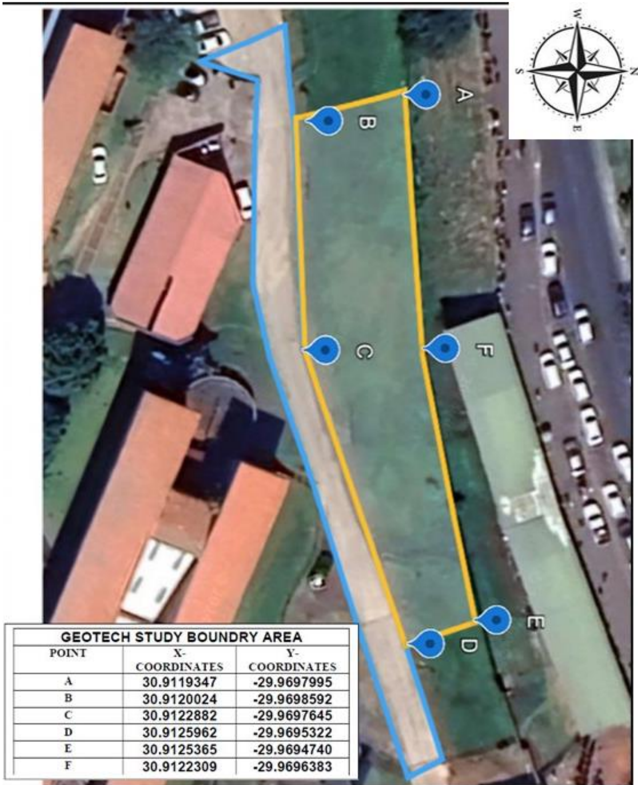
Figure 1: MUT Location 1 – 1ML Elevated Structure Proposed Geotechnical Investigation Points, Google Earth 2024
